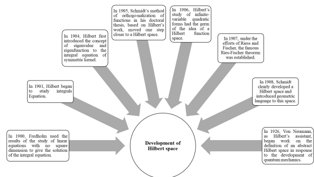
Figure 1 Development of Hilbert space
